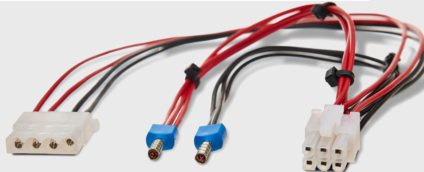
MOLEX MICROFIT 3.0, 4.96MM, HШВИ
